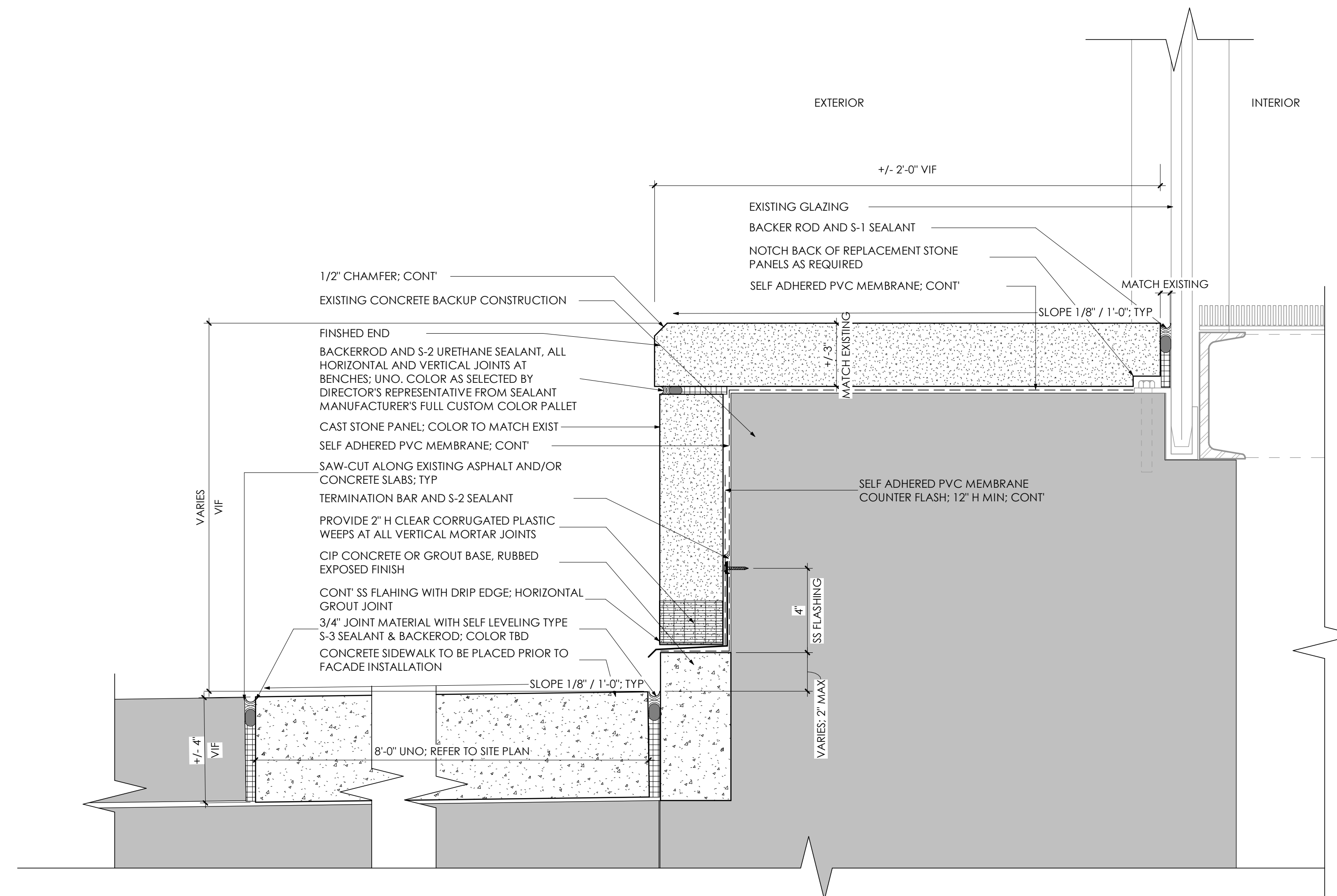
3 BENCH DETAIL 3" = 1'-0"
